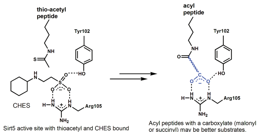
Figure 7. Schematic representation of Sirt5 active site structure with thioacetyllysine and CHES bound. 3 This structure led to the hypothesis that Sirt5 is a demalonylase or desuccinylase.
