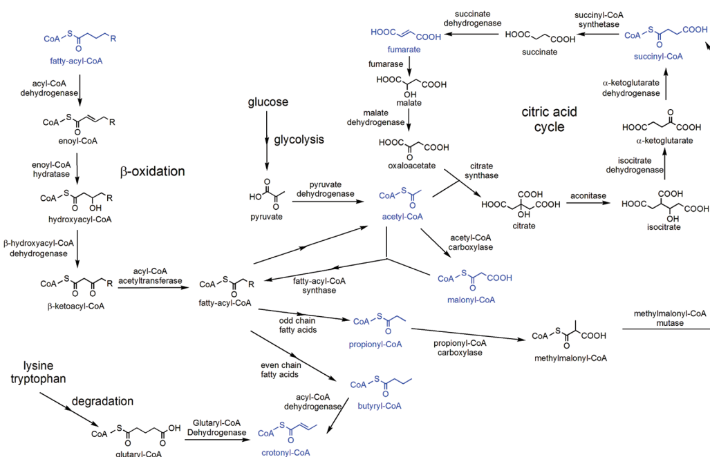
Figure 2. Metabolic pathways that provide the donors for the PTMs shown in Figure 1, except for lysine formylation.
