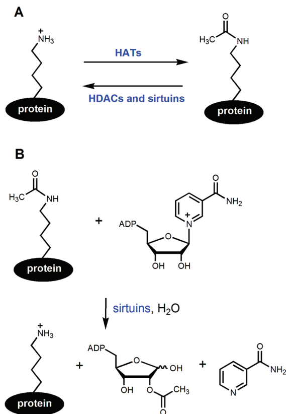
Figure 3. (A) Protein lysine acetylation and deacetylation are controlled by acetyltransferases (HATs) and deacetylases (HDACs and sirtuins). (B) The NAD-dependent deacetylation reaction catalyzed by sirtuins.
