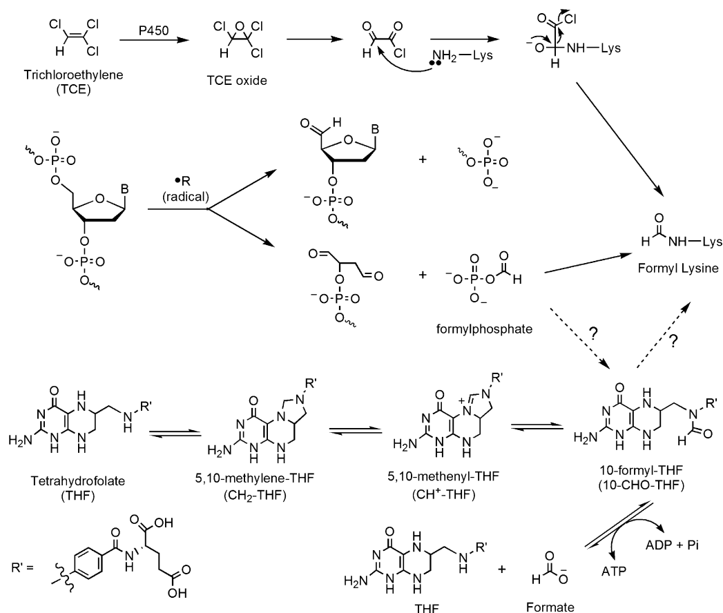
Figure 5. Different pathways for lysine formylation. Formyl-THF could be the formyl donor for a hypothetical enzymatic pathway. Dashed arrows represent possible but hypothetical steps.
