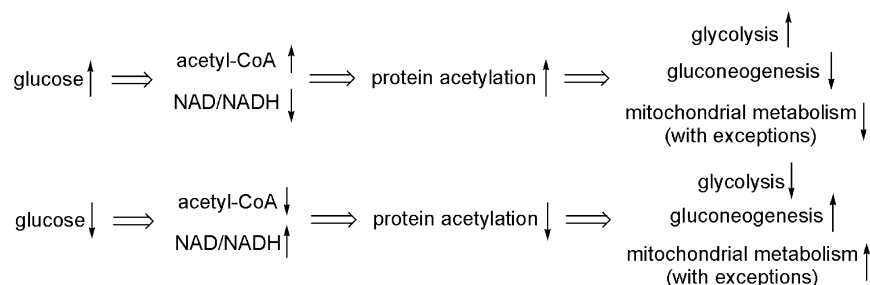
Figure 4. General model of how metabolic enzyme acetylation changes according to glucose concentration.
