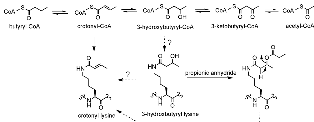
Figure 6. Possible pathways for lysine crotonylation. Dashed arrows represent possible but hypothetical steps.
