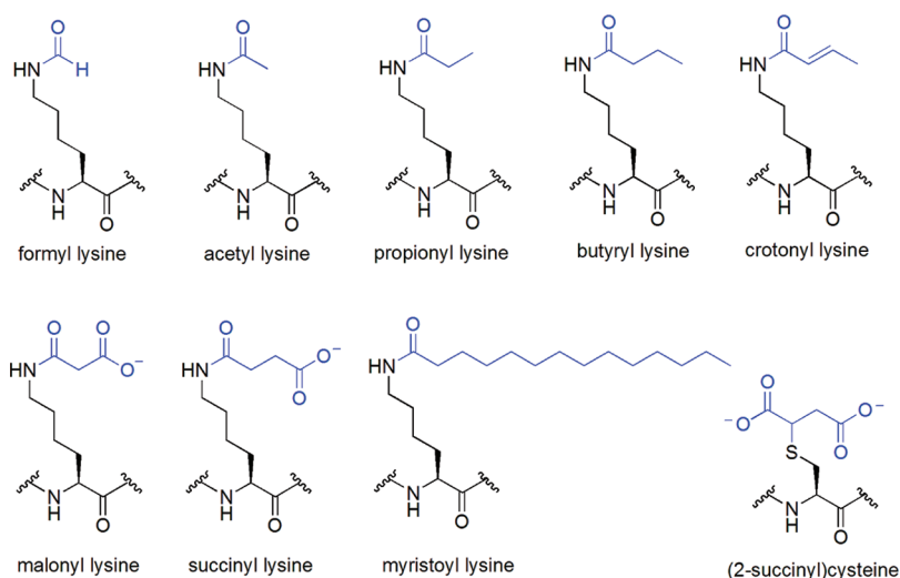
Figure 1. Structures of PTMs that will be discussed. The post-translationally added parts are colored in blue.
