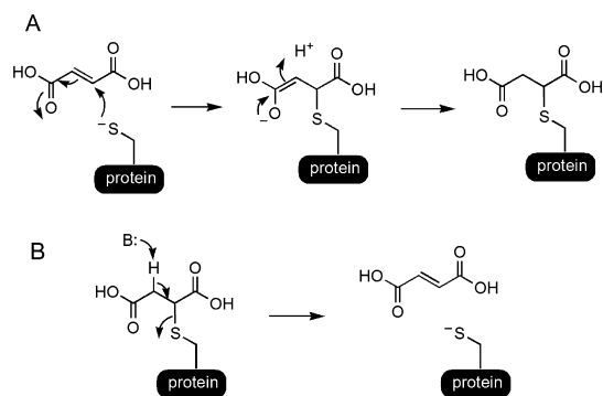
Figure 8. Cysteine succination. (A) Michael reaction for the formation of (2-succinyl)cysteine. (B) A general base can potentially promote the reversal of (2-succinyl)cysteine.
